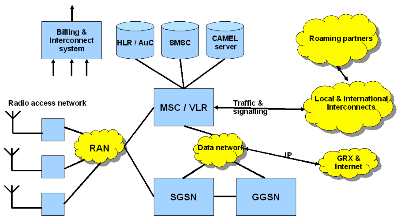
Marathon Telecom, initial network
